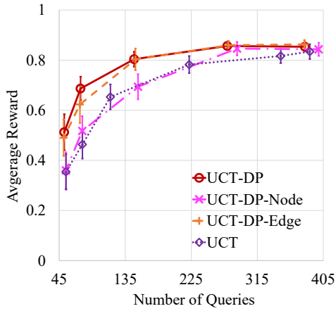
Fig. 7: Ablative studies of UCT-based approaches without default policy (UCT), with node selection default policy (UCT-DP-Node), with edge selection default policy (UCT-DP-Edge), and with both node and edge selection default policies (UCT-DP) for boost converters.
