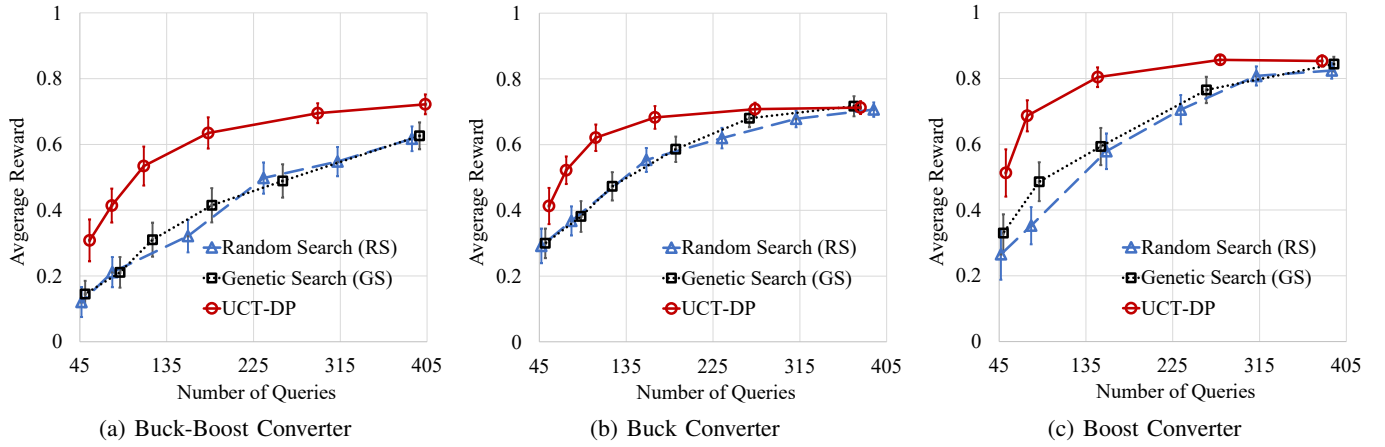
Fig. 6: Average rewards under UCT-DP vs. GS vs. RS with increasing numbers of unique queries to circuit evaluations. The x-axis shows increasing numbers of queries to circuit evaluations for unique topologies. The y-axis is the obtained reward calculated using the power efficiency and voltage conversion ratio of the best candidate circuit generated by an algorithm, averaging from 200 runs.
