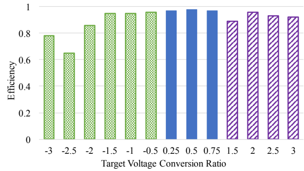
Fig. 5: Average power efficiencies of power converters generated by the proposed framework for custom design tasks with increasing voltage conversion ratios. From left to right in different colors and shades, the target converter types are buck-boost, buck, and boost.
